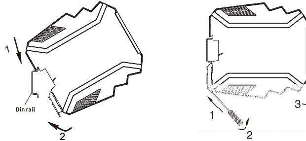
Fig.2: Mounting method
